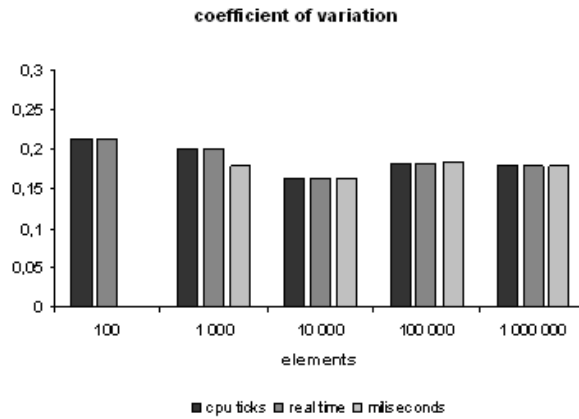
Fig. 5. Coefficient of variation for the number of CPU clock cycles, real-time and milliseconds that were obtained during performed tests
